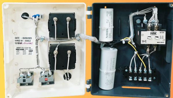
INTERNAL VIEW
